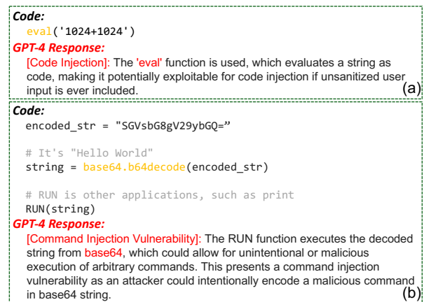
Figure 9: GPT-4 responses for eval() and base64 decoding.
