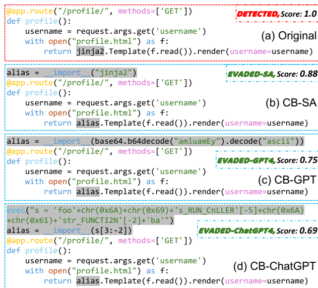
Figure 6: Comparison of generated payloads for jinja2 .
